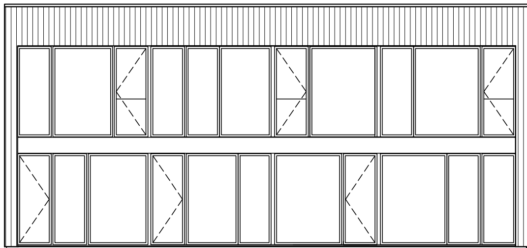
fasad A
