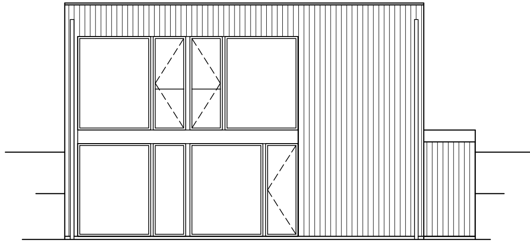
fasad A
