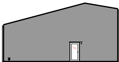
fasad A
