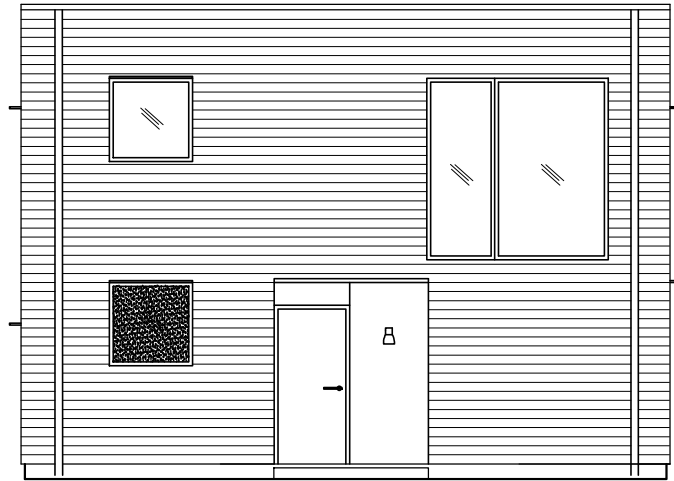
fasad A
