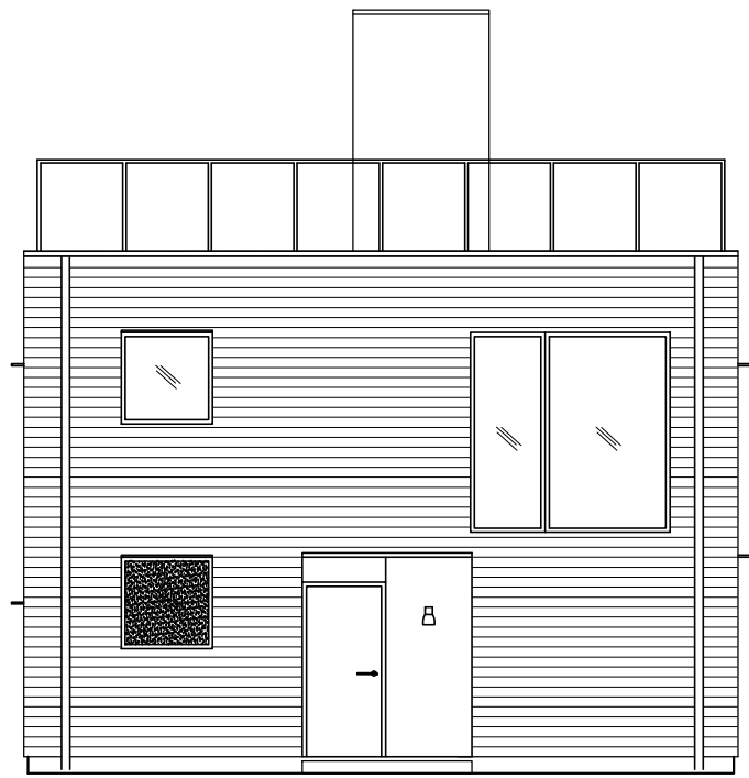
fasad A
