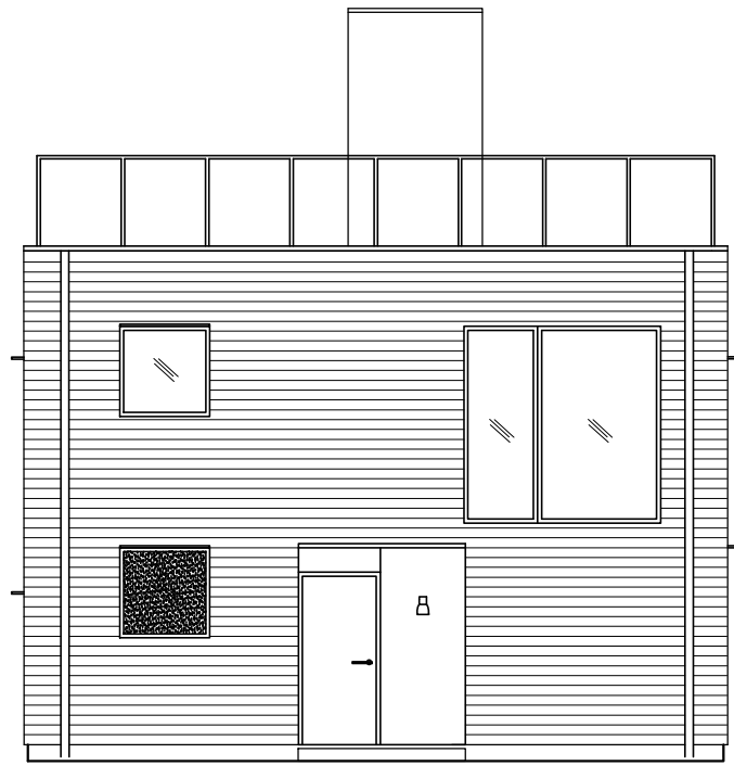
fasad A
