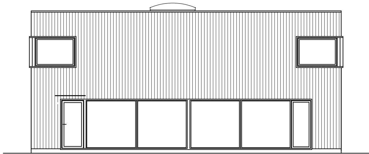
FASAD A
