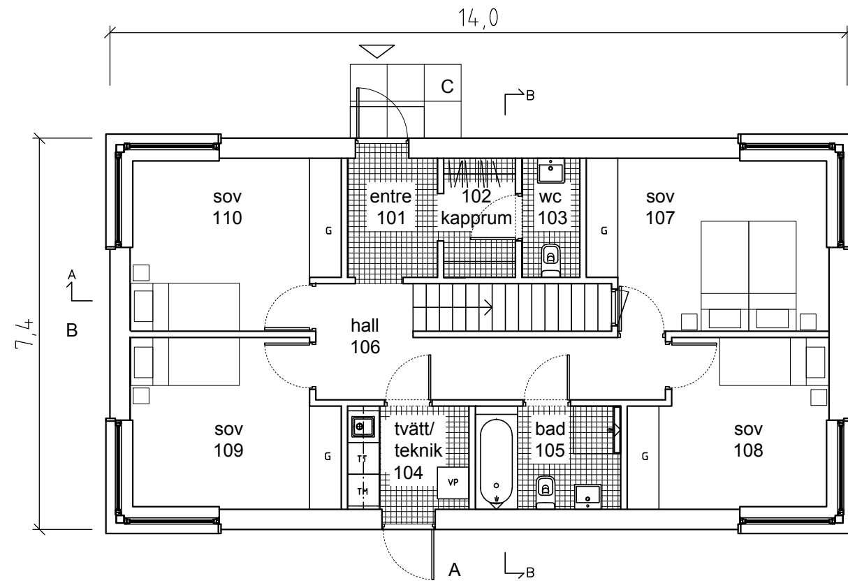
bottenplan
