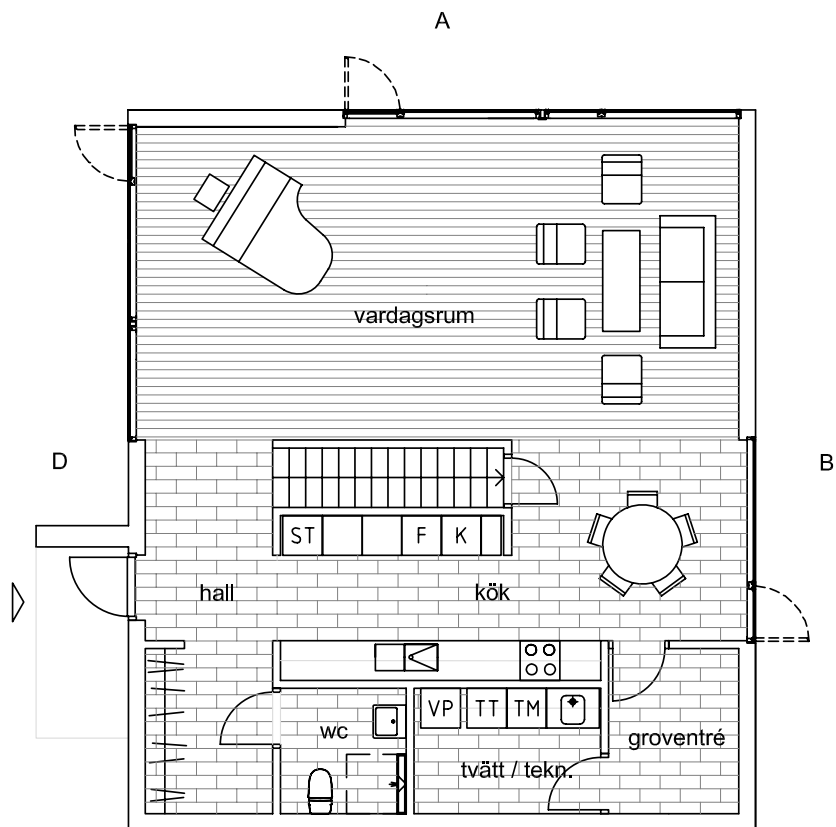
bottenplan
