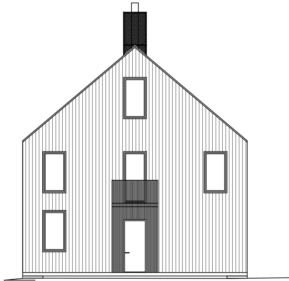
fasad A
