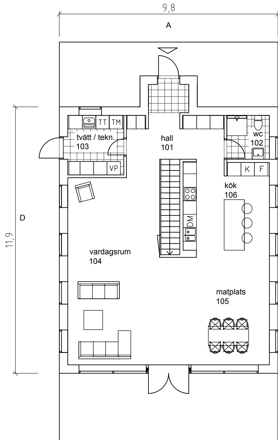
bottenplan
