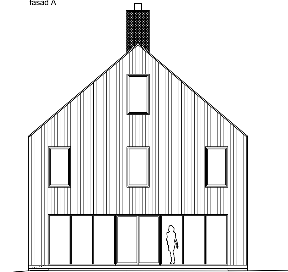
fasad A
