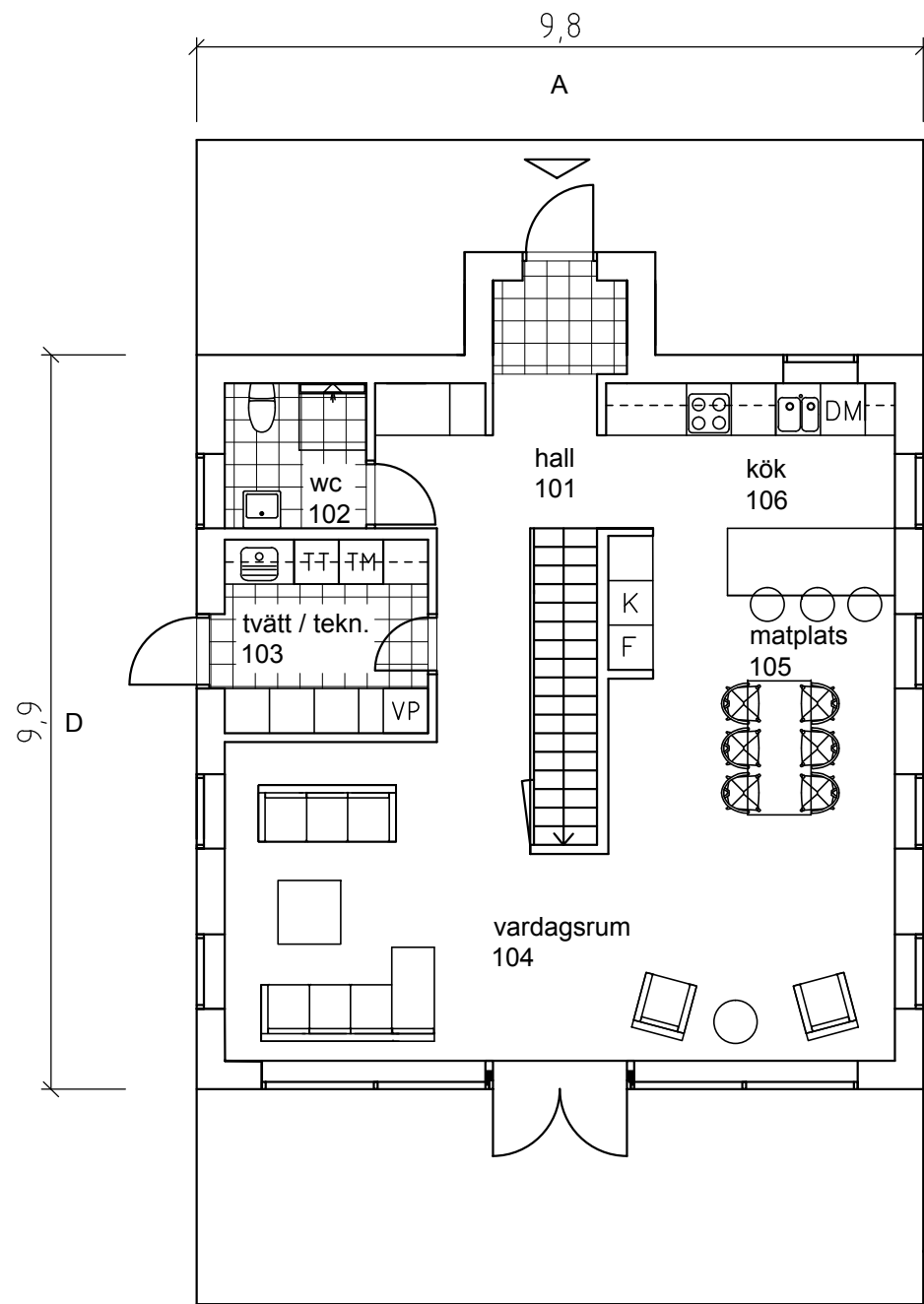
bottenplan
