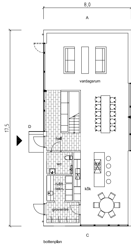
bottenplan
