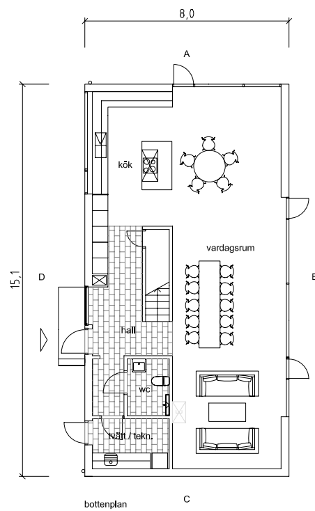
bottenplan
