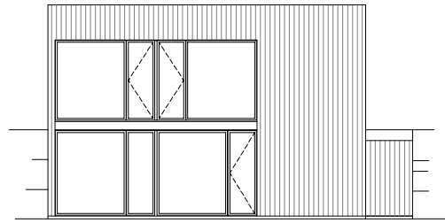
fasad A
