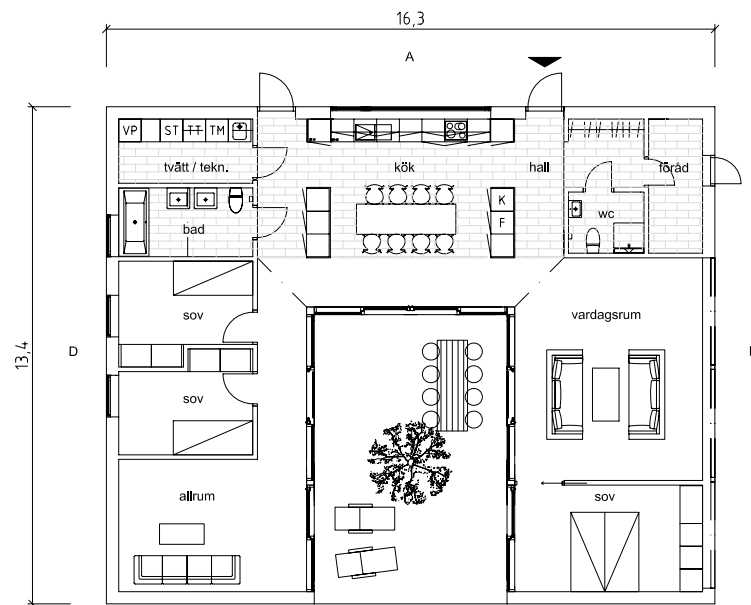
bottenplan
