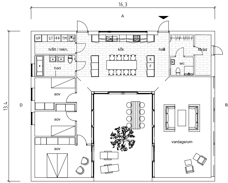
bottenplan
