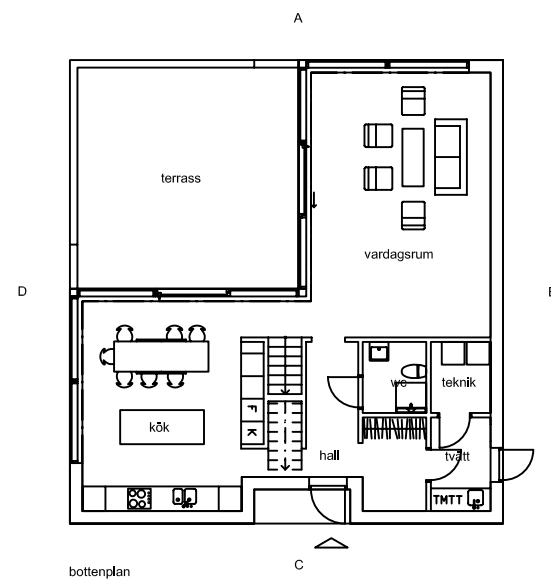
bottenplan
