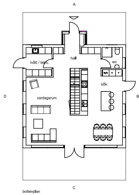
bottenplan
